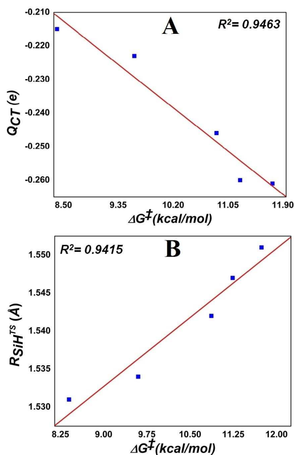
Figure 4. \Delta G^\ddagger vs. (A) Q_{CT} and (B) R_{SiH^{TS}} in Si–H insertions.
